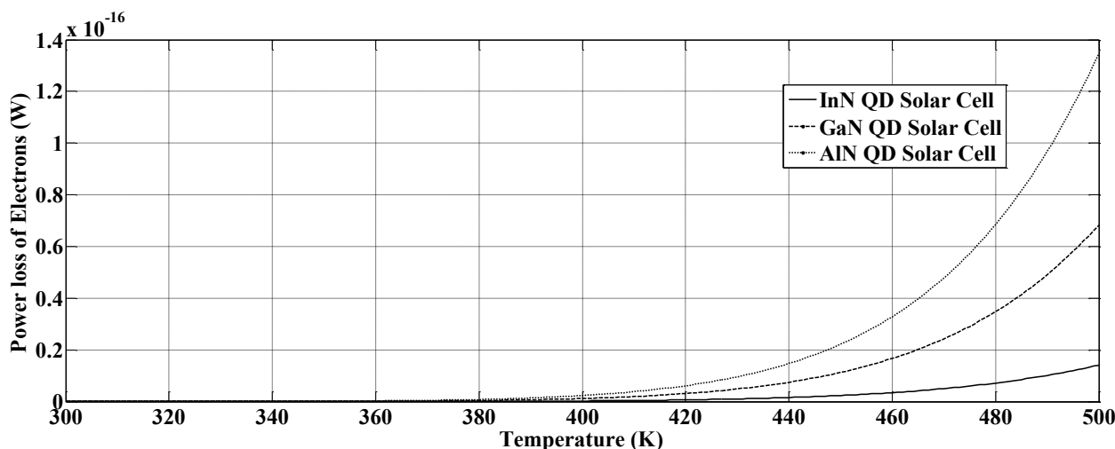
Fig. 4: Power loss of electrons in QDSC at different temperature conditions using InN (Solid curve), GaN (Dashed curve) and AlN (Dotted curve) QD in the active layer
