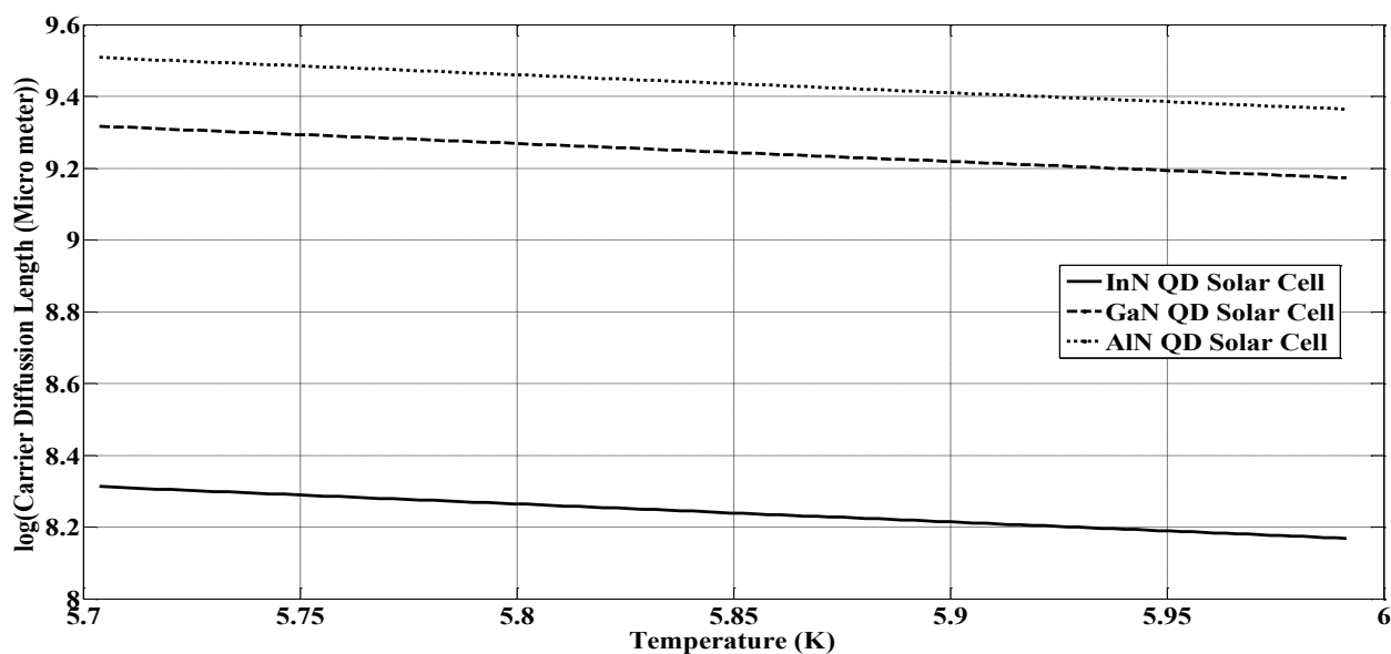
Fig. 3. Temperature dependence of diffusion length of carriers in QDSC using InN (Solid curve), GaN (Dashed curve) and AlN (Dotted curve) QD in the active layer.
