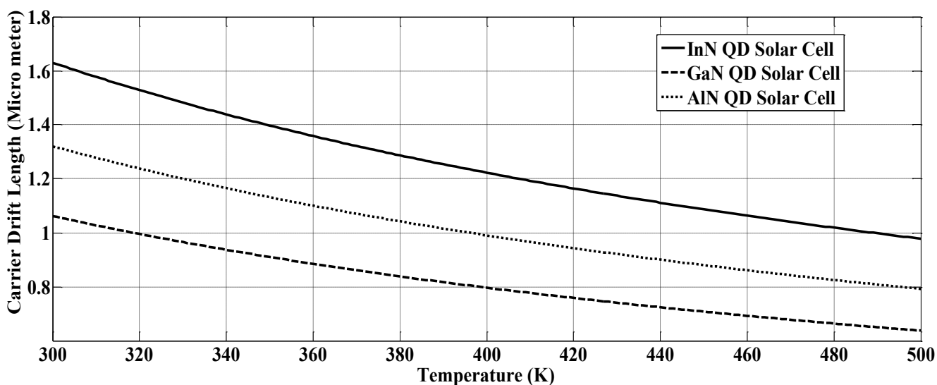
Fig. 2. Temperature dependence of drift length of carriers in QDSC using InN (Solid curve), GaN (Dashed curve) and AlN (Dotted curve) QD in the active layer.
