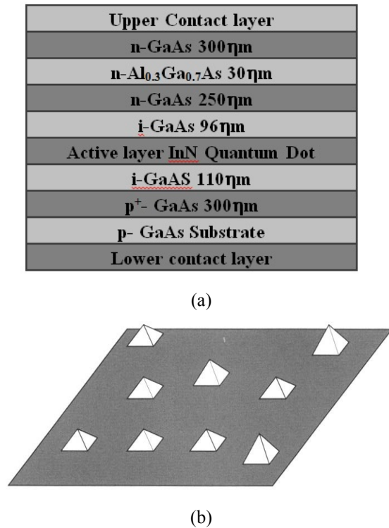
Fig. 1. (a) Schematic layer structure of InN QDSC (b) InN QD array
